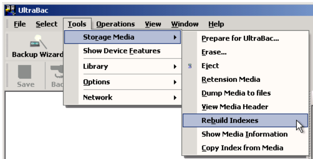
Fig. 26 - Rebuilding the Continuous Image Protection index.
