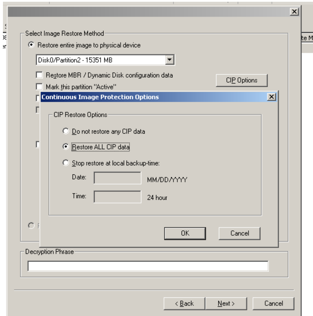
Fig. 27 - Continuous Image Protection restore options.
